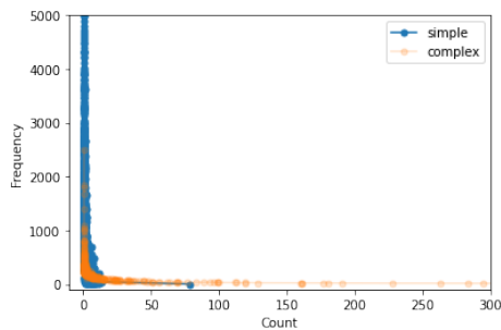
(c) CLASSIFICATION
