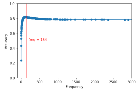
(a) READABILITY
