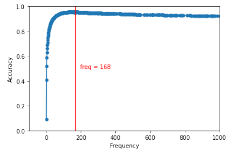
(c) CLASSIFICATION
