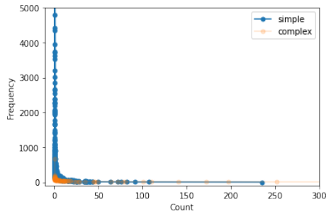
(b) CLUSTER
