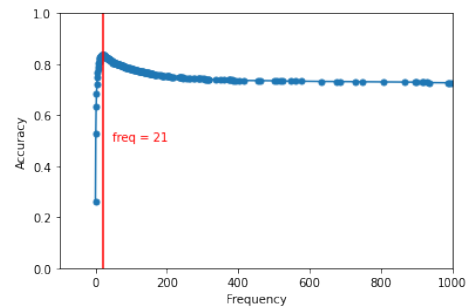
(b) CLUSTER
