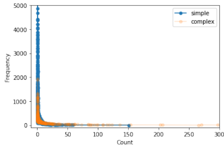
(a) READABILITY
